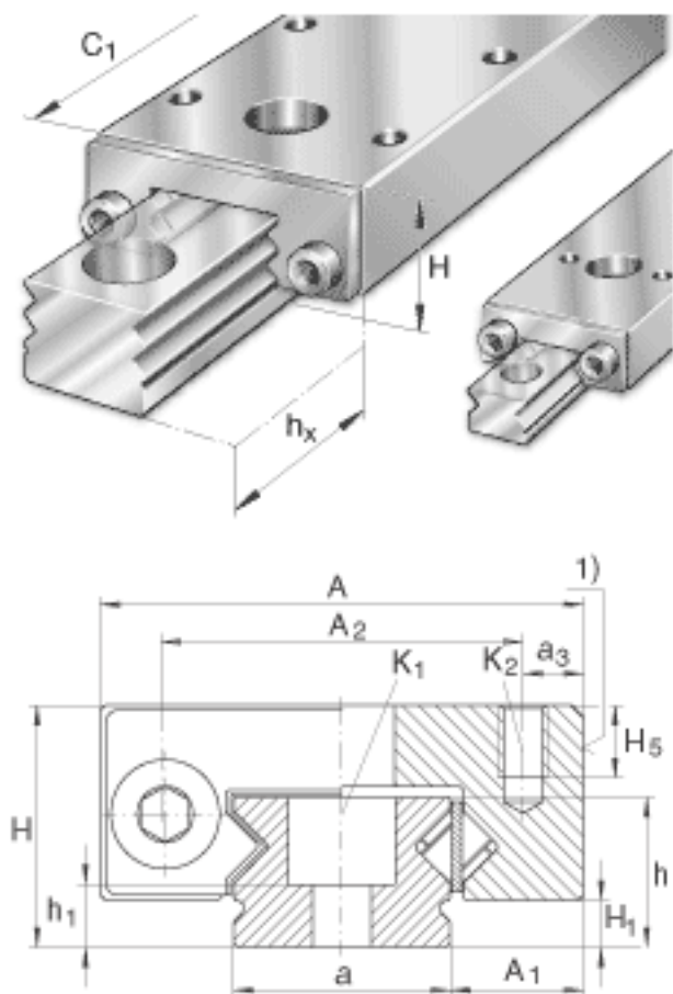
INA RMWE09A-RB/129x.../86图片
